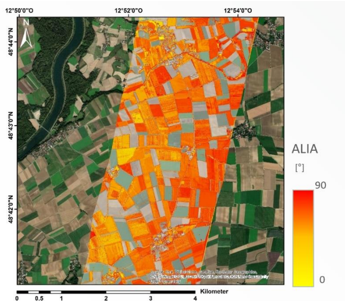
Figure 18 Exemplary map of ALIA, generated using the hybrid processor of the EnMAP-Box Agri-tools: Neural network trained over PROSAIL data base (agricultural region of Neusling (Bavaria, Germany).
