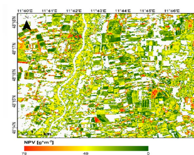
Figure 22 Exemplary map of NPV biomass, based on hybrid retrieval method using ARTMO MLRA-toolbox: GPR trained over PROSAIL-PRO simulated data base.
