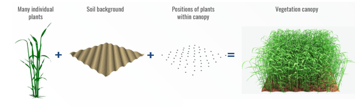
Figure 6a Structure of a vegetation stand.
