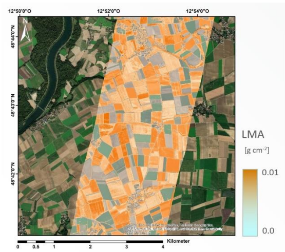
Figure 14 Exemplary map of LMA, generated using the hybrid processor of the EnMAP-Box Agri-tools: neural network trained over PROSAIL data base (Neusling, Bavaria, Germany).
