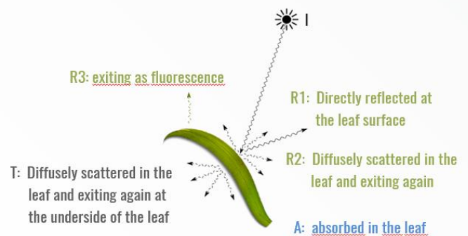
Figure 2 Interaction of radiance with leaf. Adapted from Berger et al. (2021) Spaceborne Imaging Spectroscopy of Agricultural Systems (HYPERedu slide collection)
