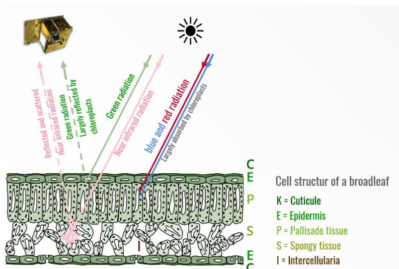
Figure 3 Leaf cell structure.
